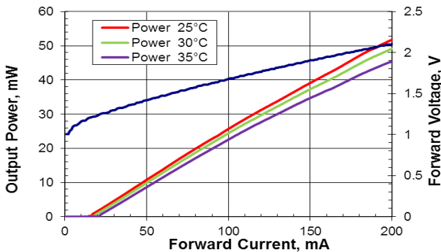
Light-Current-Voltage Characteristics
