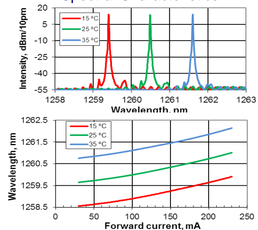
Spectral Characteristics
