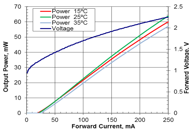
Light-Current-Voltage Characteristics
