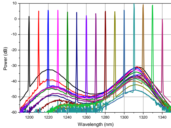
Optical spectra @ 800mA (res. 0.5 nm)
