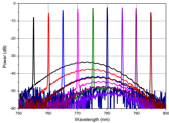
Optical spectra @ 250mA (res. 0.2 nm)
