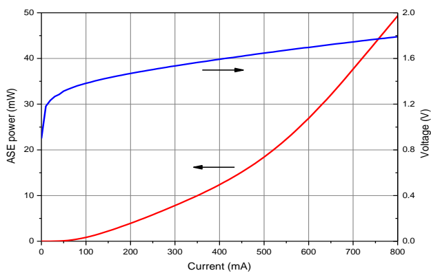
Light-Current-Voltage Characteristics
