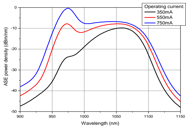
Spectral Characteristics
