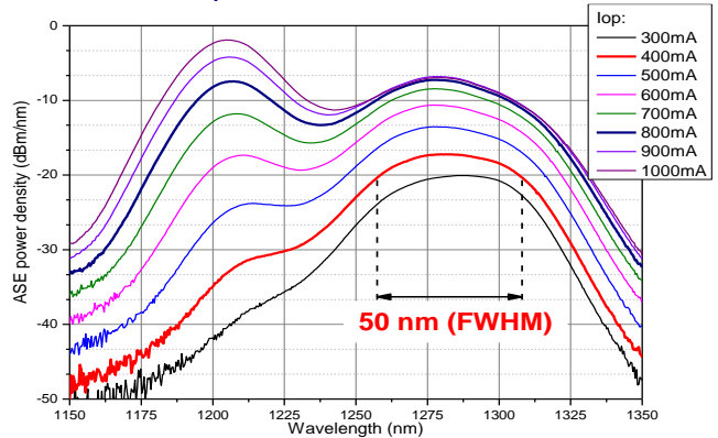
Spectral Characteristics
