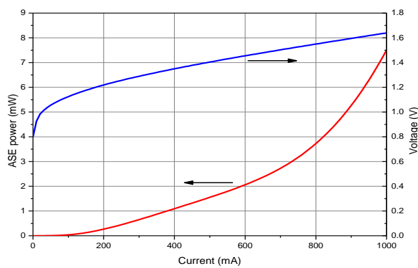
Light-Current-Voltage Characteristics
