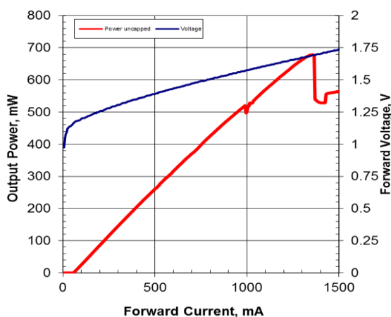
Light-Current-Voltage Characteristics
