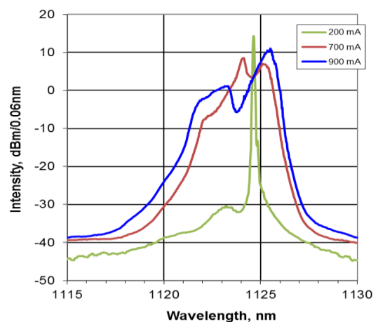
Spectral Characteristics
