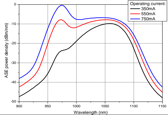
ASE Spectra (no input signal)
